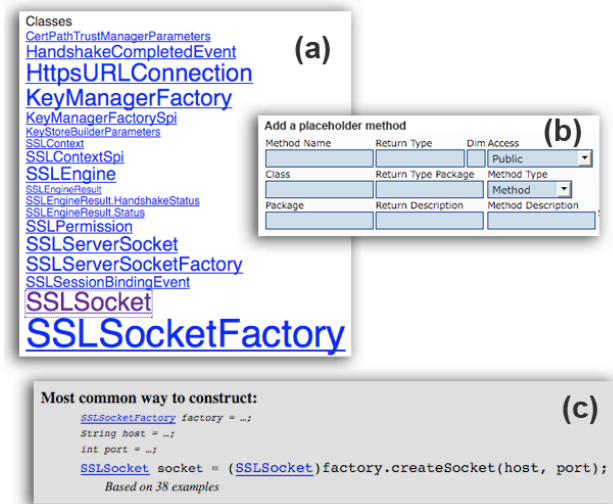
Figure 1. Novel features of the Jadeite documentation system. Font sizes are varied based on usage data (a); common methods of class construction (c) are automatically determined; and users can add new placeholder classes or methods (b) to stand in for expected parts of an API.
