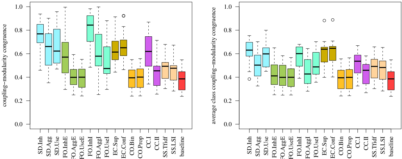
Figure 2: Coupling-modularity congruence and average class coupling-modularity congruence.
